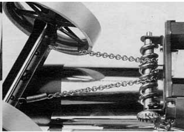
Illustration 31a ONLY FOR TRACTION ENGINES
